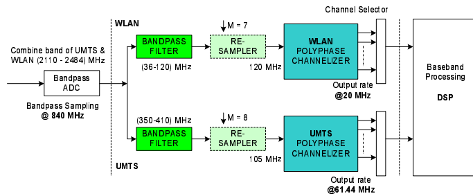
Fig. 7. System block diagram having re-samplers prior to UMTS and WLAN channelizers.
