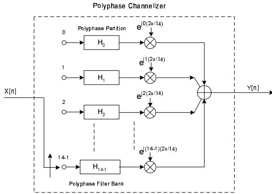
Fig. 12. UMTS channelizer
