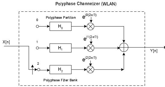
Fig. 10. WLAN channelizer.
