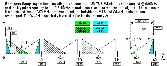
Fig. 9. The combined spectrum of UMTS and WLAN is bandpass sampled at 630MHz, and the resulted aliases in the Nyquist zone. WLAN alias is spectrally inverted.
