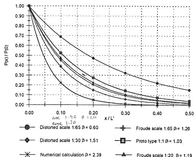
Figure 2 Pore pressure attenuation in the breakwater.
