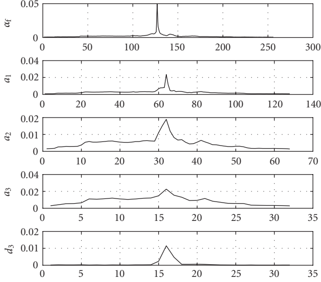
FIGURE 8: The part of the tree of variances of \alpha_f[n] , as defined in the scheme. The figure starts with the original signal. The second plot is h , the third is hh , the fourth is hhh , and the last one is hhg .
