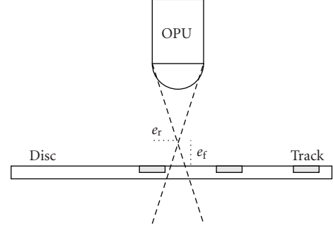
FIGURE 1: The focus distance, e_f , is the distance from the focus point of the laser beam to the reflection layer of the disc; the radial distance, e_r , is the distance from the center of the laser beam to the center of the track.
