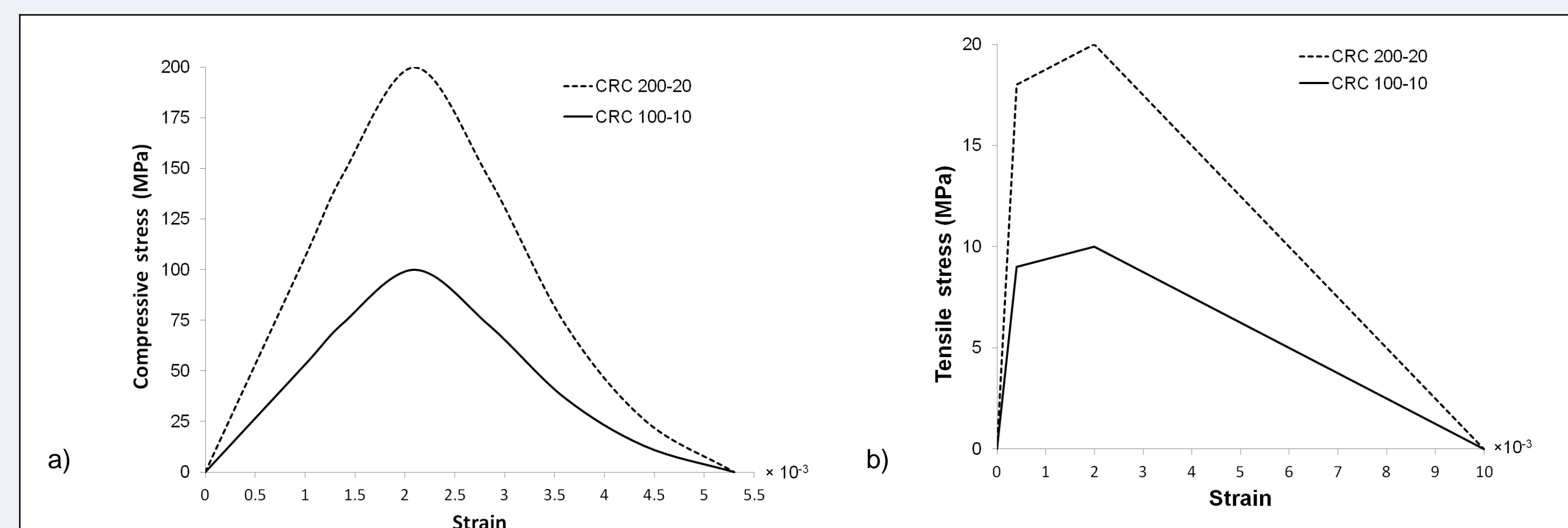
Figure 4: Stress-strain curves for CRC: a) compressive behaviour; b) tensile behaviour.
