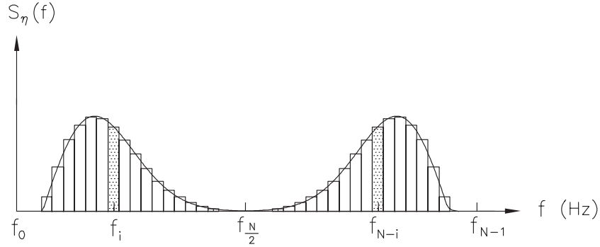
Figure 5.17: Variance spectrum.
