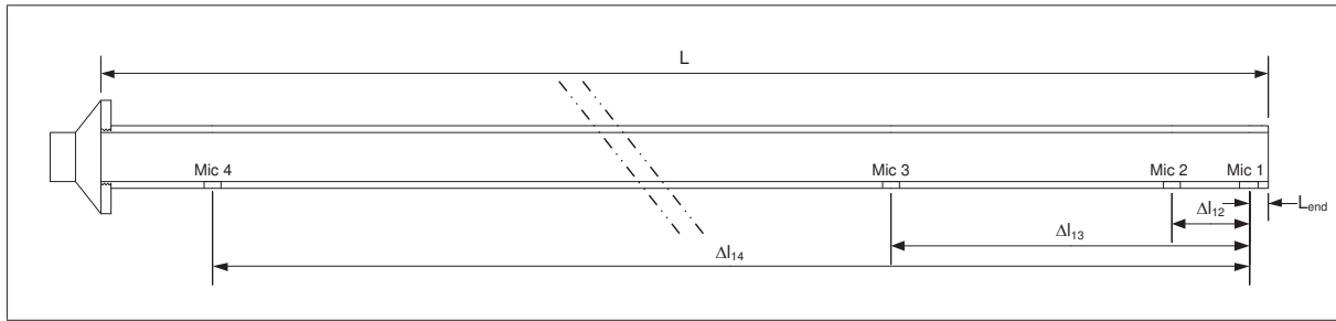
Figure 1. Impedance tube. Dimensions can be found in Table I.
