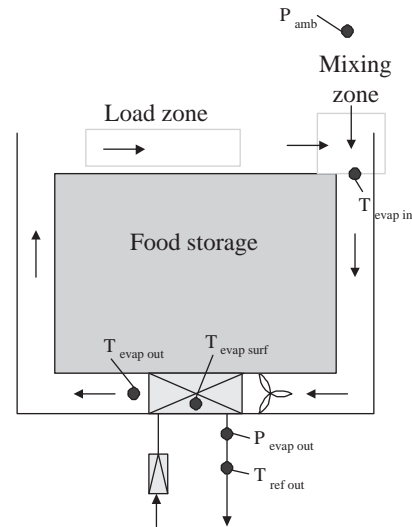
Fig. 1. A simplified display cabinet in the supermarket
