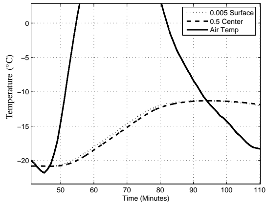
(a) h=5 \text{ W}/(m^2.K)
