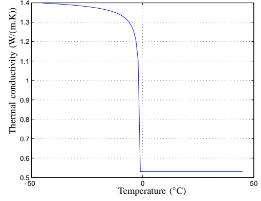
Fig. 6. Dependence of thermal conductivity with temperature
