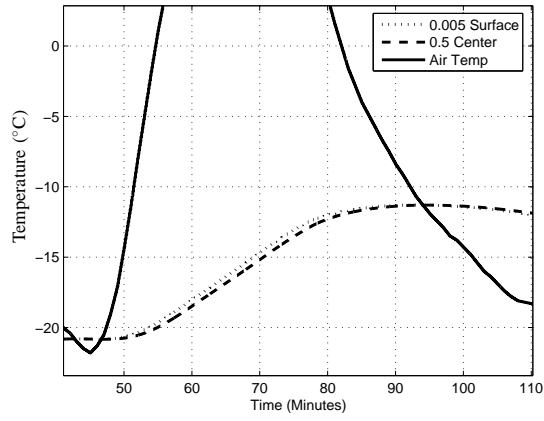
(a) h=5 \text{ W}/(\text{m}^2.\text{K})
