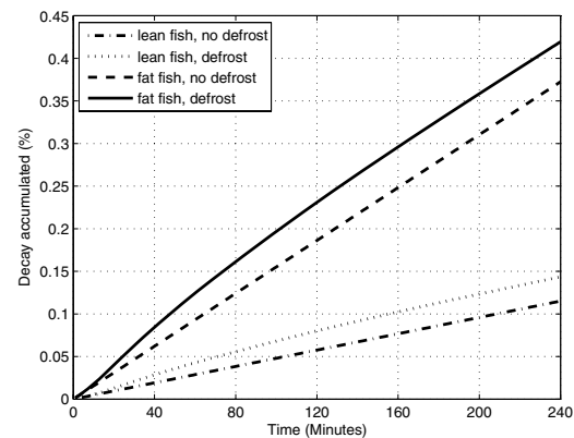
Figure 13: frozen fish decay- defrost vs. no defrost
