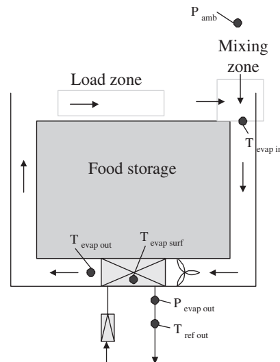
Figure 1: Simplified display cabinet in supermarket
