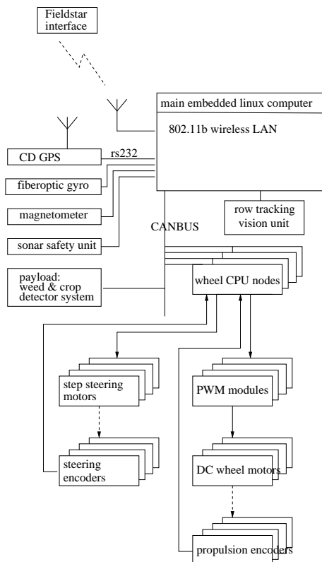
Figure 3: Sketch of electrical layout
