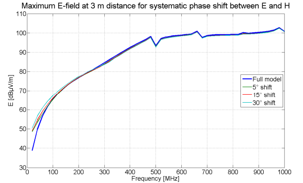
Figure 11: Systematic phase across the PCB, model 1.
