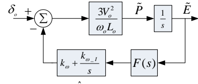
Fig. 7. Block diagram relating \hat{E} to \delta_o
