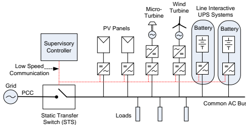
Fig. 1. Microgrid structure.
