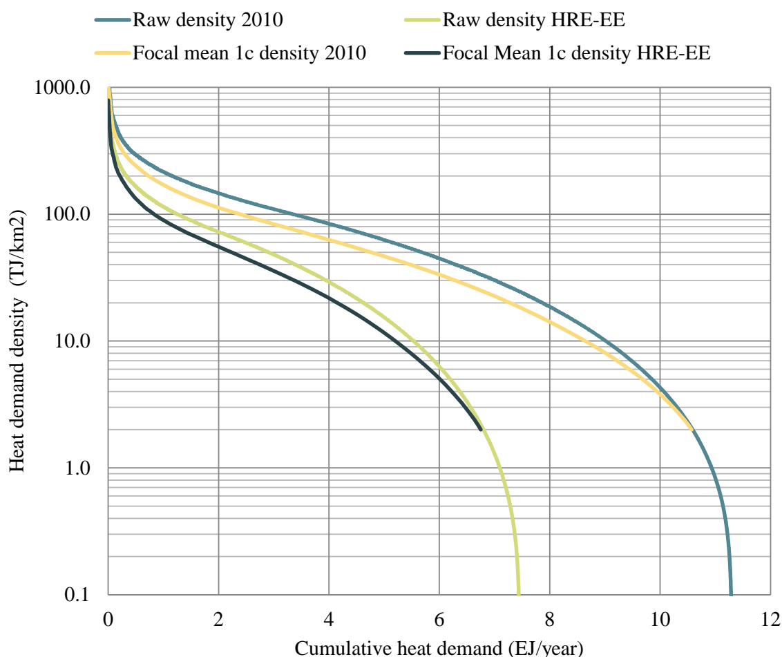
Figure 15: Cumulative heat demand according to the European Heat Atlas in 2010 and in the Heat Roadmap Europe Energy Efficiency (HRE-EE) scenario, by two different types of heat density calculations. Raw density is the density calculated in each square kilometre cell, while Focal mean density is the density if calculating the mean of a cell and its neighbourhood cells, thereby levelling out density values but resulting in more coherent prospective district heating areas.
