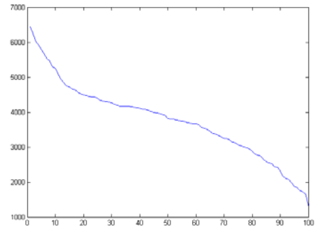
Fig. 4. Generalized Hankel Singular Value( \gamma_i )
