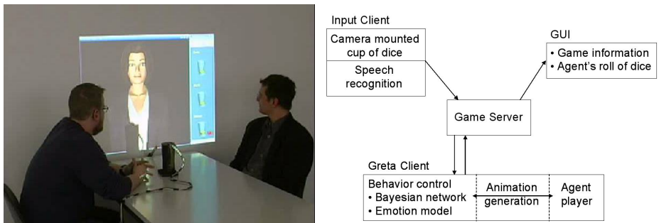
Fig. 1. The setting (left) and the system architecture (right). The agent is projected to the wall at the end of the table, thus sitting together with the other players around the table. Between the human players, the CamCup and the microphone are visible.
