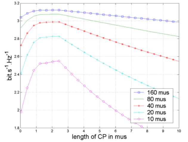
Figure 4: Capacity vs. CP length for different useful OFDM symbol lengths, PDP=PedB, SNR=20dB.
