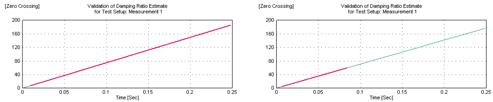
Figure 4. Natural frequency identification by zero-crossing counting without (left) and with (right) deterministic signal. Mode at 354 Hz. Deterministic signal at 374 Hz.
