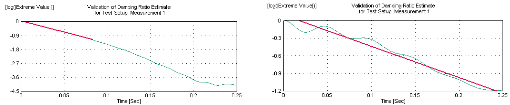
Figure 5. Damping ratio estimation from the decay of the correlation function without (left) and with (right) deterministic signal. Mode at 354 Hz. Deterministic signal at 374 Hz.
