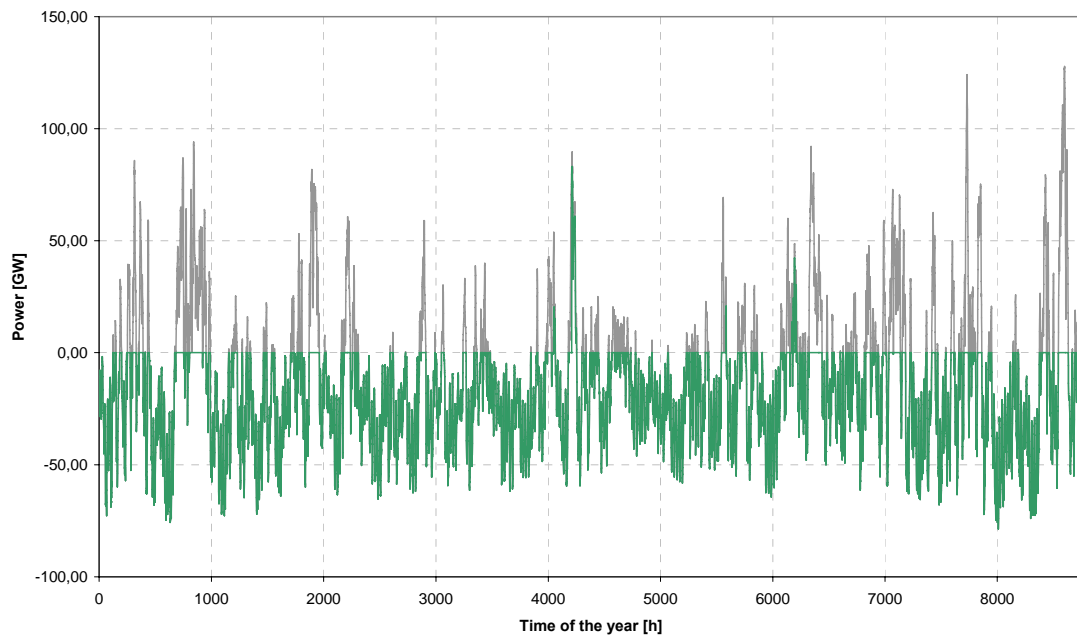
Figure 3-24: Scenario II: Balanced with contribution of Demand Side Management
