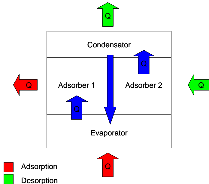
Figure 5-7: Adsorption Chiller
