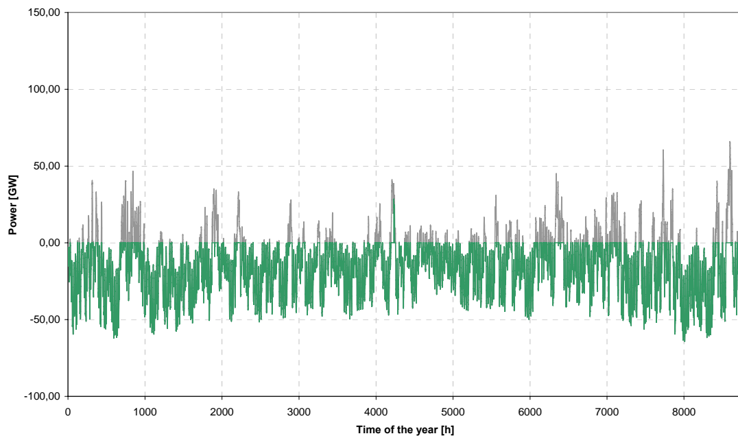
Figure 3-26: Scenario III: Balanced with contribution of Demand Side Management
