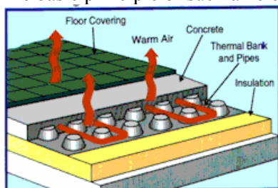
Figure 11-10: Floor-elements /TEAP/
