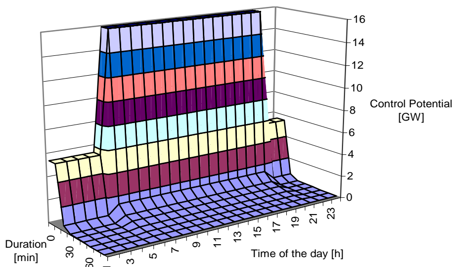
Figure 3-8: Negative Control Potential of air-conditioning units (Source: /Stadler 2005/)
