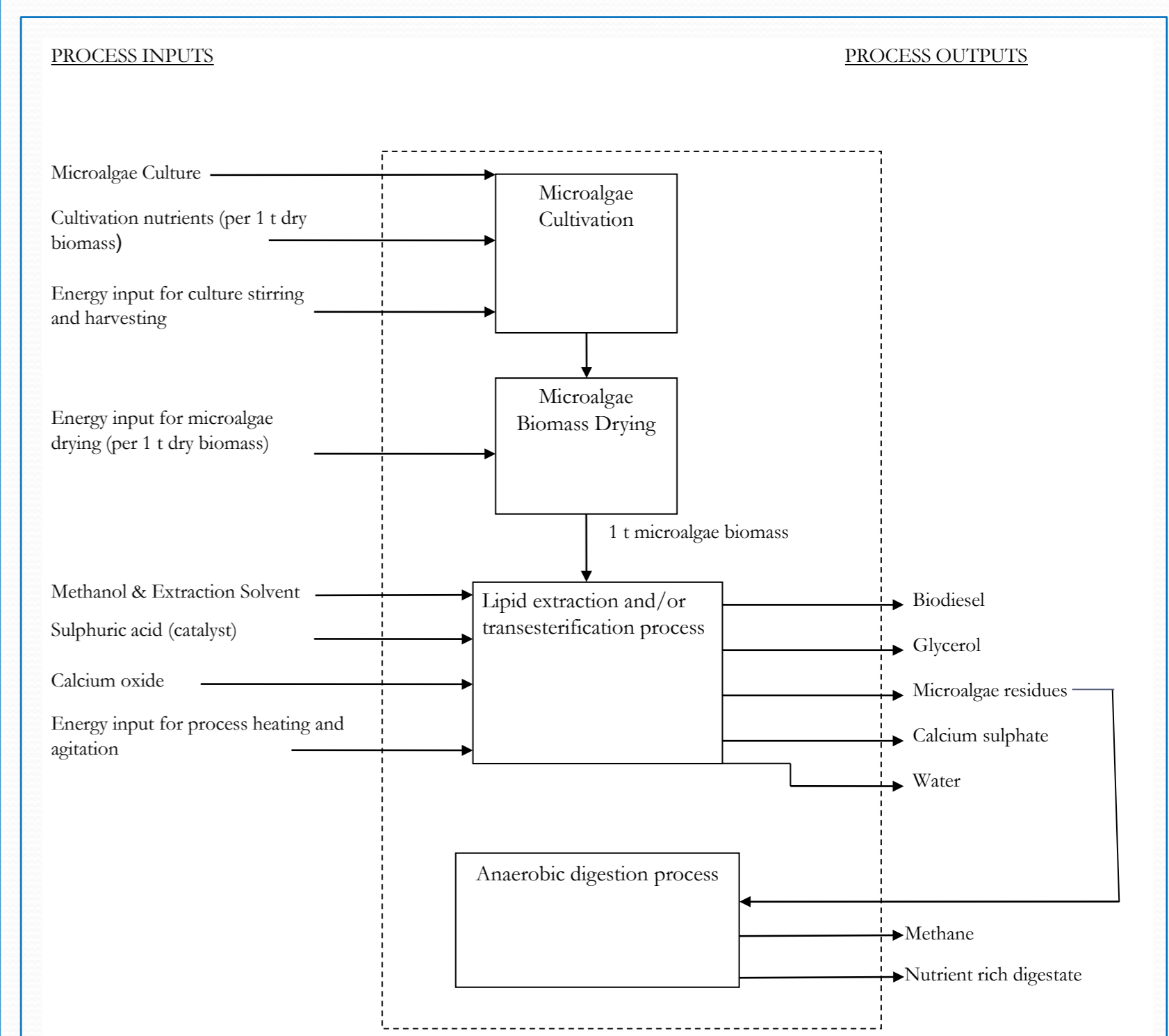
Fig. 1. The system boundary (dashed lines) and material and energy flows considered in this study.
