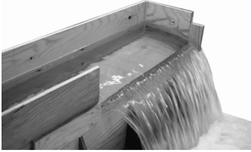
Figure 5 Physical model of side weir
