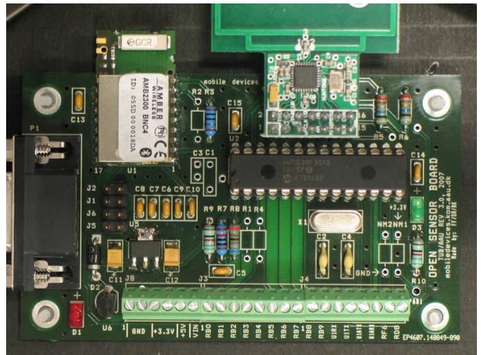
Fig. 2. A picture of the opensensor board version 3.0.
