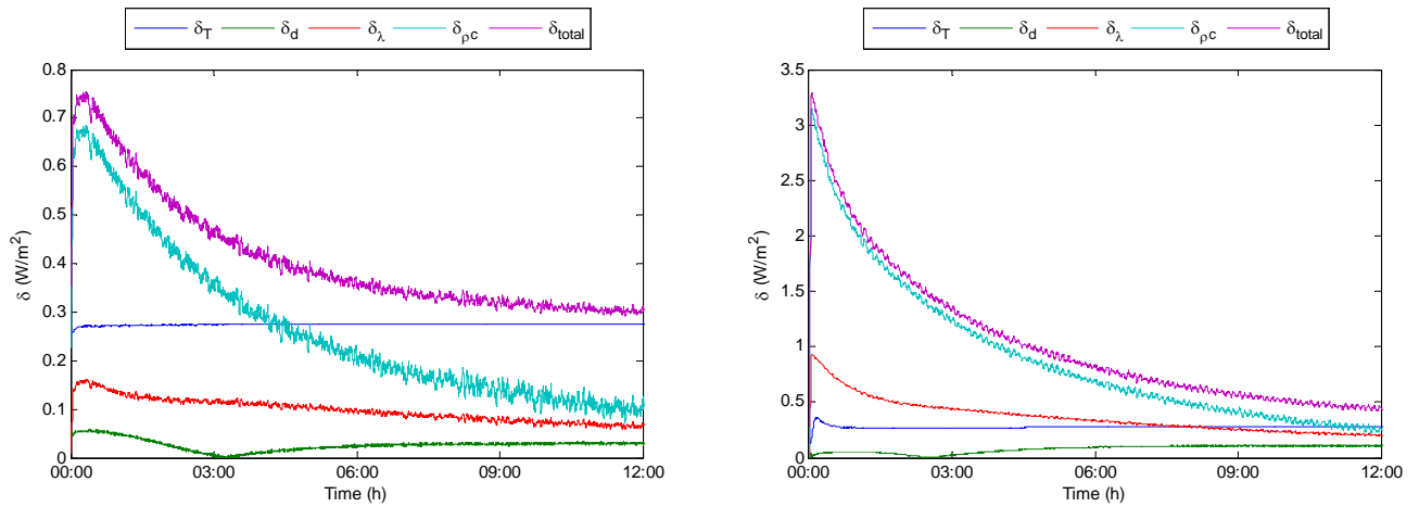
Figure 22. Uncertainty in the conductive heat flux at the ceiling due to different input parameters; left: small heat flux (experiment no. 4, position 8); right: high heat flux (experiment no. 10, position 8).
