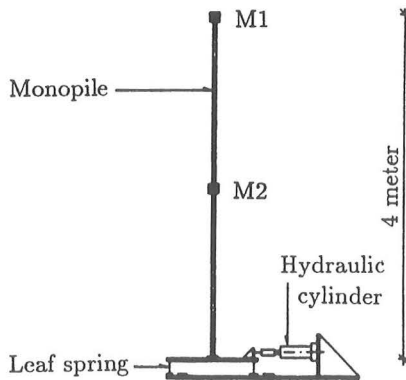
Figure 2. Monopile structure.
