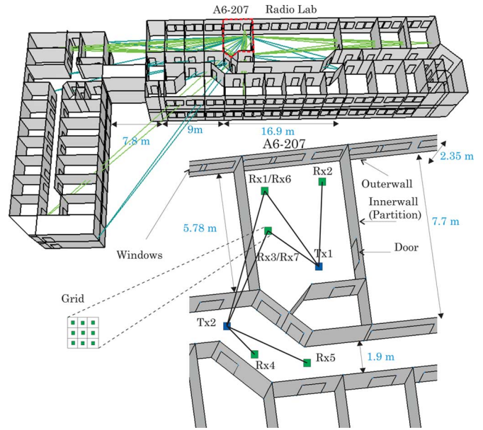
Fig. 3. Three-dimensional view of the APNet building with 1st order reflection.
