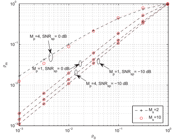
Fig. 2. The target outage probability at primary node \rho_m in presence of cognitive radio versus the outage probability in absence of the secondary system for different values of average interference SNR at primary receiver and different number of primary BS and secondary BS antennas M_p and M_s , respectively.
