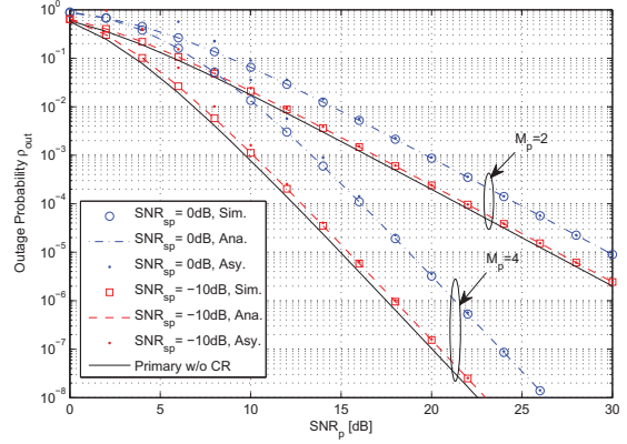
Fig. 1. Outage probability in the primary system as a function of the received primary SNR, i.e., \text{SNR}_p when M_s = 2 and R_p = 1 bits/s/Hz. The systems with different number of M_p and \text{SNR}_{\text{sp}} are compared.
