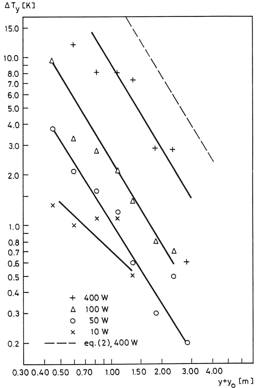
Fig. 9. Temperature difference \Delta T_y versus distance y+y_0 . Circular plate d = 356.8 mm.
