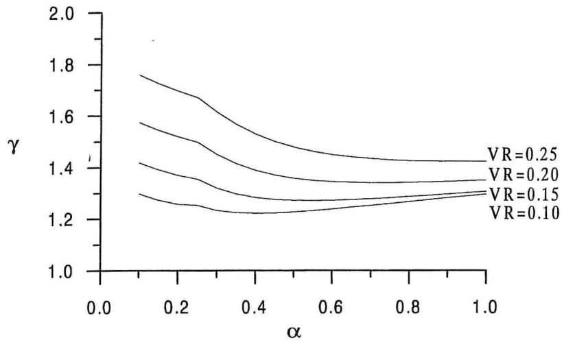
Figure 11.6. Partial safety factor for imposed load and \beta_t=4.3 .
