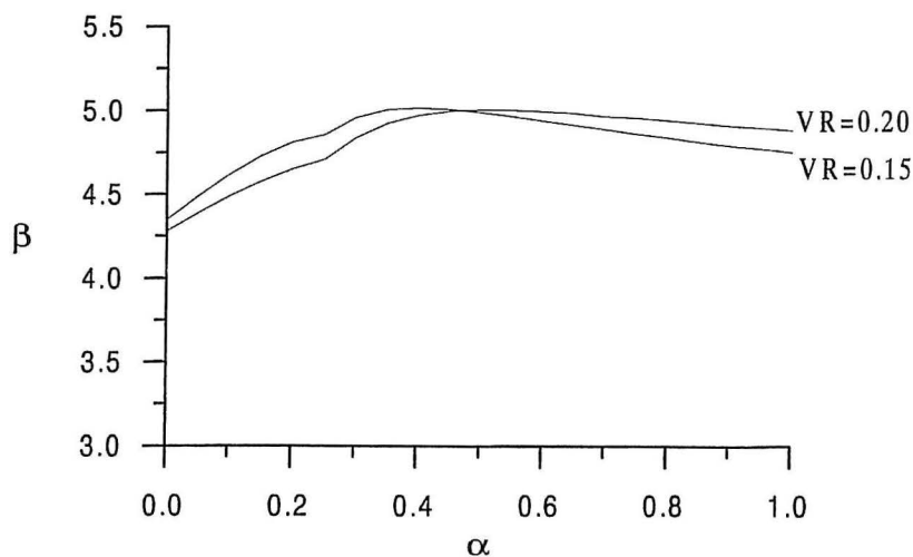
Figure 11.2. Reliability index for imposed load.
