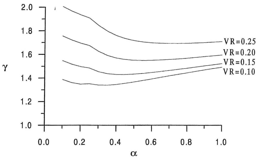
Figure 11.4. Partial safety factor for imposed load and \beta_t=4.8 .
