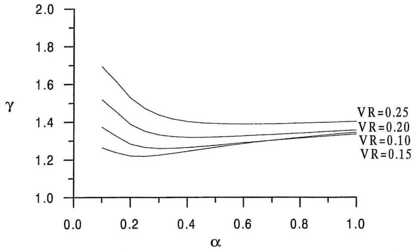
Figure 11.5. Partial safety factor for environmental load and \beta_t=4.3 .
