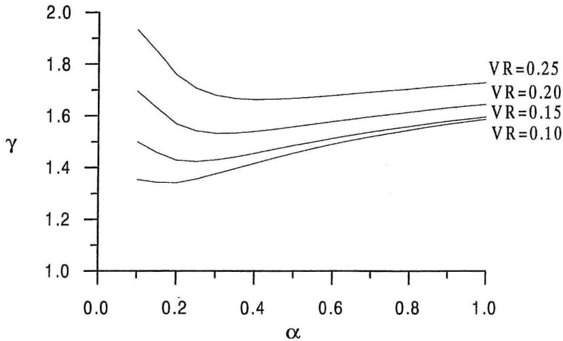
Figure 11.3. Partial safety factor for environmental load and \beta_t=4.8 .
