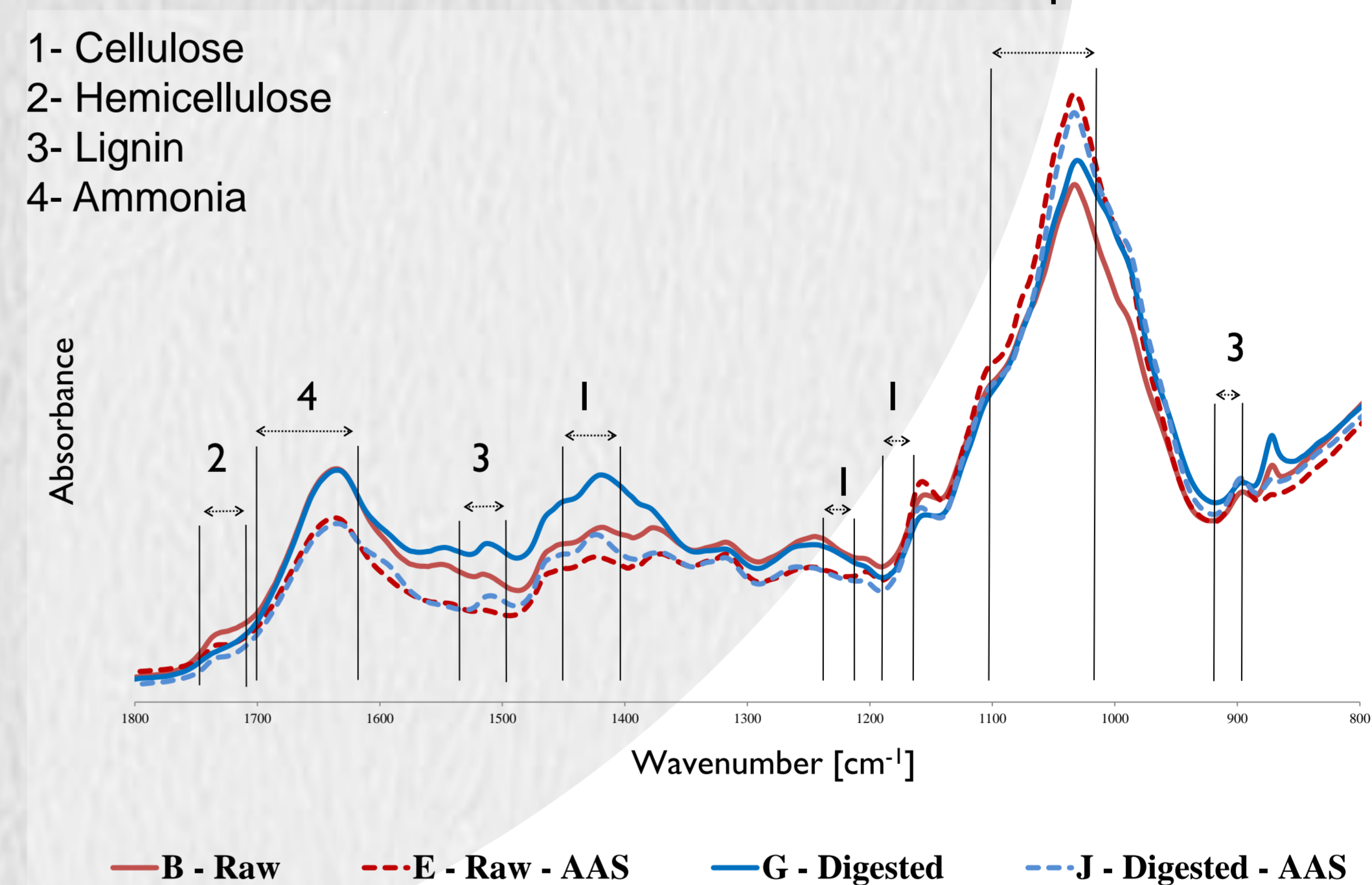
ATR-FTIR analysis
