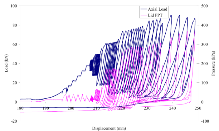
Figure 20. Load-displacement curve of test 14 ( Kelly 2006b ).
