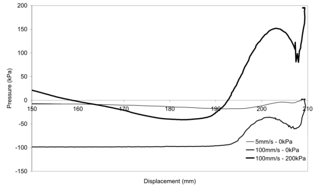
Figure 17. Pressures beneath the lid of the caisson during ultimate tensile loading in Redhill 110 sand (Kelly et al. 2006b).
