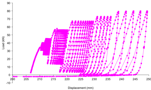
Figure 7. Cyclic loading followed by pull-out (Kelly 2003).
