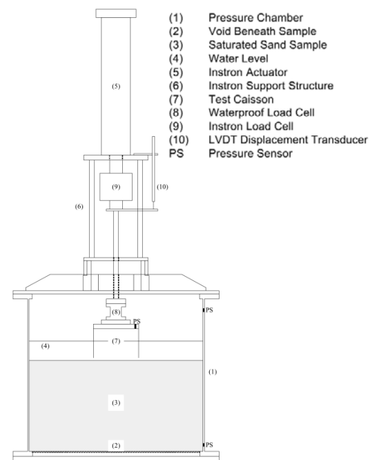
Figure 6. Pressure chamber (Kelly 2003).
