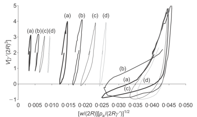
Figure 23. Comparison suction and push installation: installations by suction a) field test, b) 150 mm diameter caisson installed by suction, c) 200 mm diameter caisson installed by pushing, d) 150 mm diameter caisson installed by pushing. Kelly (2006a).
