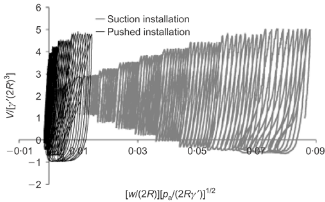
Figure 10. Cyclic loading after suction and pushed installation (Kelly et al. 2006a).
