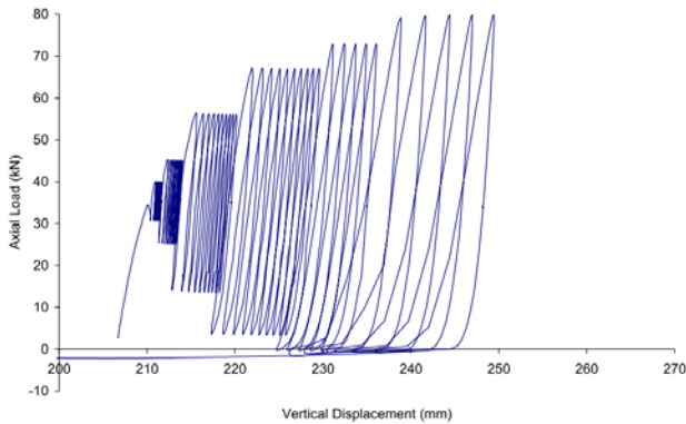
Figure 8. Cyclic loading in Redhill 110 loaded at a rate of 1Hz (Kelly et al. 2006b).
