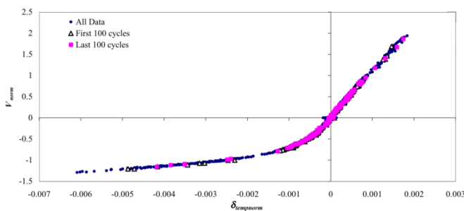
Figure 21. Long cycle response (Byrne 2000).
