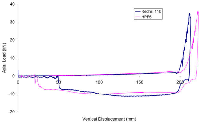
Figure 16. Pull-out response of large displacement test (Kelly et al. 2004).
