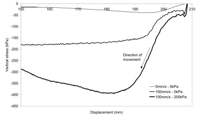
Figure 18. Ultimate tensile loading in Redhill 110 sand (Kelly et al. 2006b).
