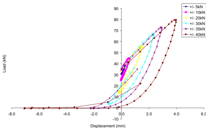
Figure 19. Cyclic loading carried out at different amplitudes ( Kelly 2003 ).
