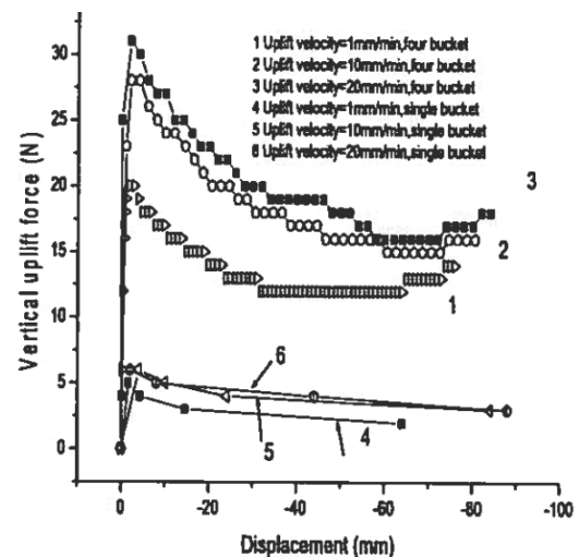
Figure 11. Load-displacement curve of single and four-caisson model under uplift loading (Lu et al. 2009).
