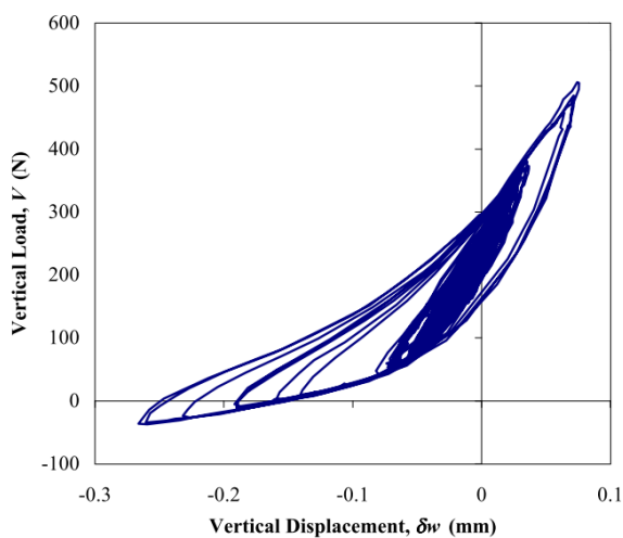
Figure 3. Asymmetrical cyclic response (Byrne 2000).
