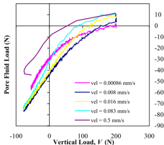
Figure 4. Pore pressure development (Byrne 2000).
