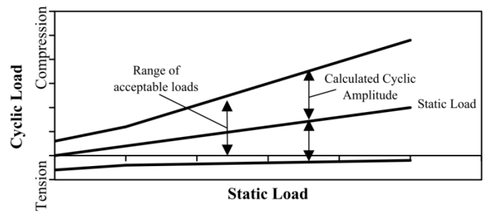
Figure 22 cyclic bearing capacity (Bye et al. 1995).
