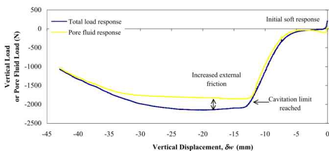
Figure 5. Response of high displacement pull-out (Kelly 2003).
