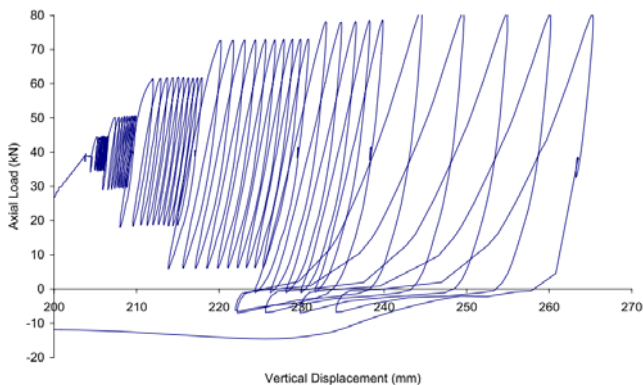
Figure 9. Cyclic loading in Oakamoor HPF5 loaded at a rate of 0.1Hz (Kelly et al. 2006b).
