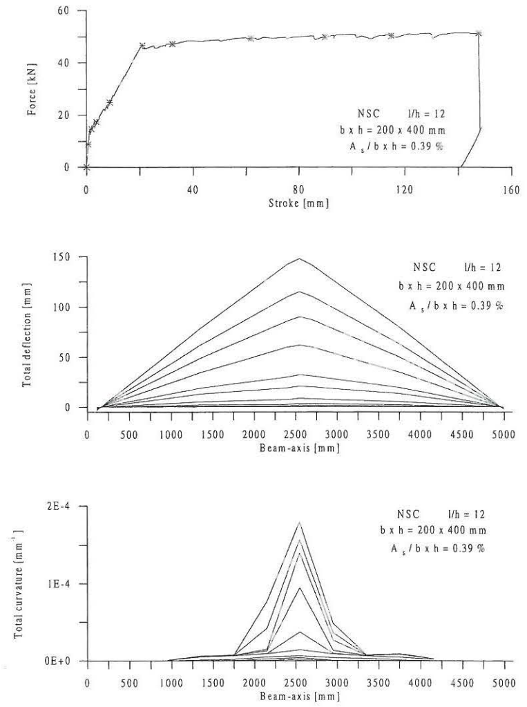
Figure A7. Load-deflection curve (top), vertical distribution (mid) and distribution of curvature (bottom) along the beam axis for a normal strength concrete beam (200 × 400 × 4800 mm) with a reinforcement ratio of 0.39 %. The load levels are marked with asterisk (top).
