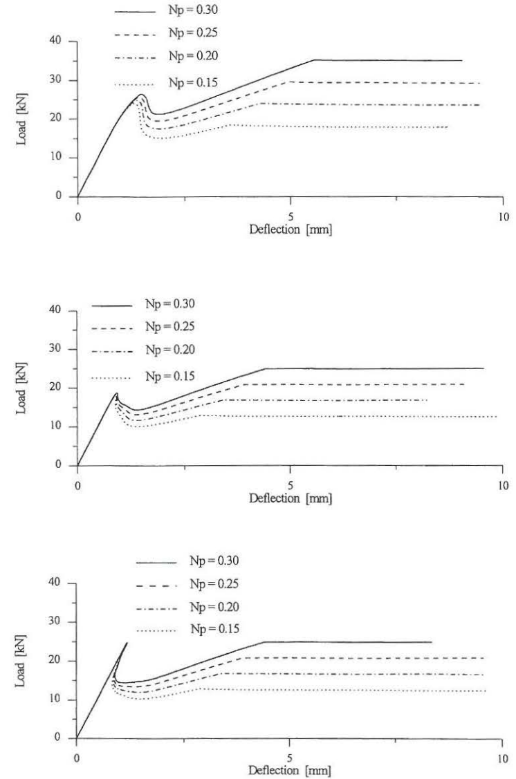
Figure B7. Variation of the failure response with brittleness number N_P for the 200 \times 400 \times 4800 mm beam. Top: Normal strength concrete with linear softening. Middle: Normal strength concrete with bi-linear softening. Bottom: High strength concrete with bi-linear softening.
