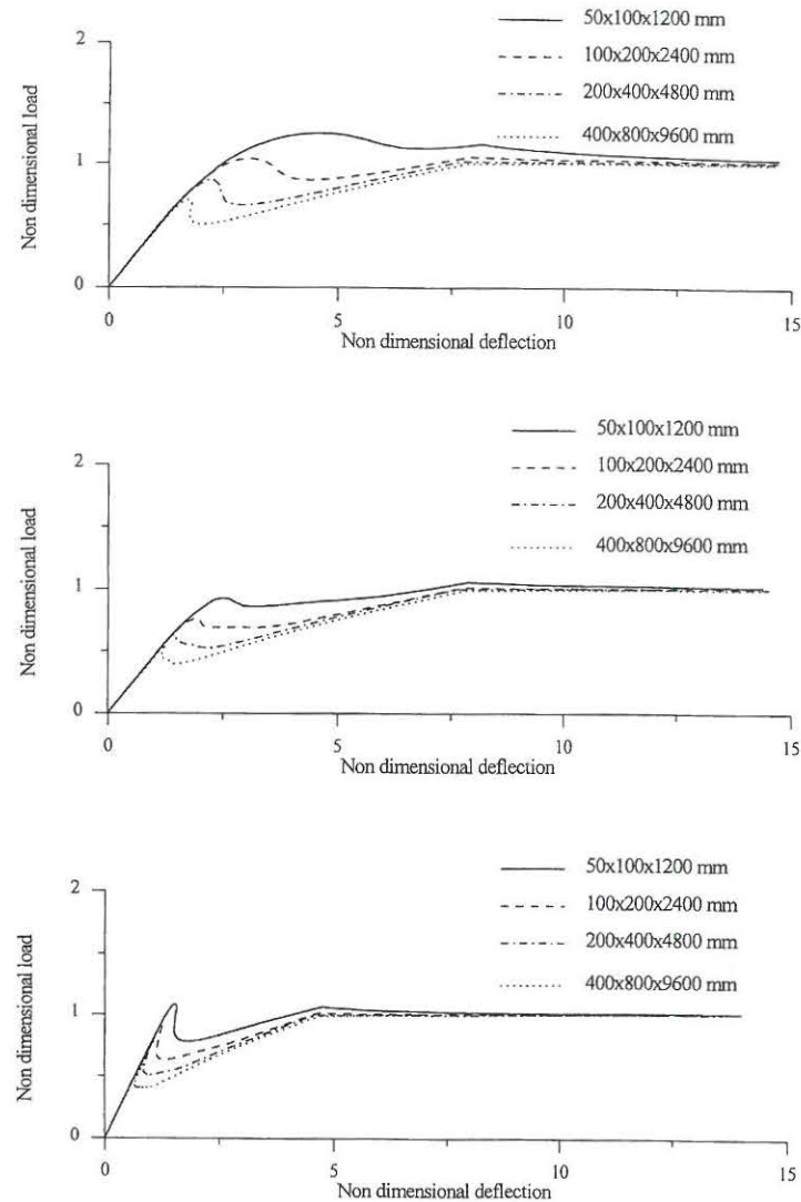
Figure B6. Size effects on the failure response for constant reinforcement ratio \varphi = 0.25\% . Top: Normal strength concrete with linear softening. Middle: Normal strength concrete with bi-linear softening. Bottom: High strength concrete with bi-linear softening.
