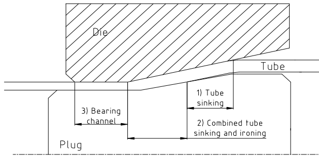
Figure 1 Sketch of the tube drawing process with a floating plug
