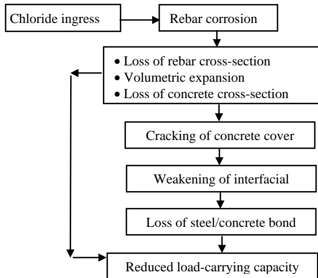
Figure 1. The physical effect of corrosion.
