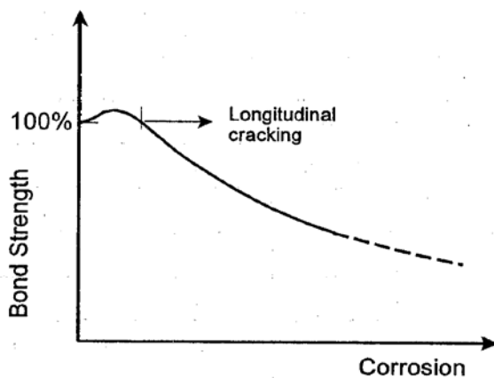
Figure 3. Schematic illustration of the variation in bond strength with corrosion (taken from FIB [4]).
