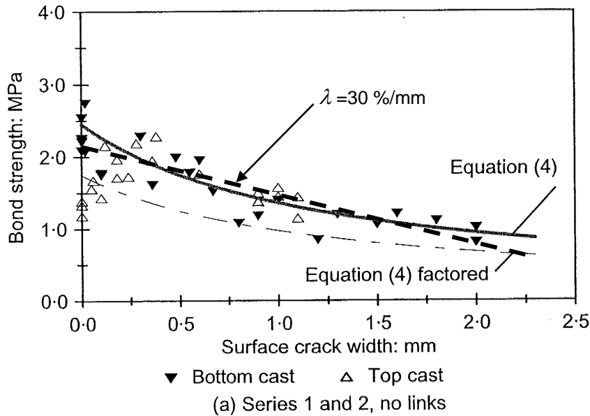
Figure 6. Relationship between bond strength f_{bond} and longitudinal crack width w_{crack} (from the top part of Fig. 8 in Cairns, Du & Law [22]).
