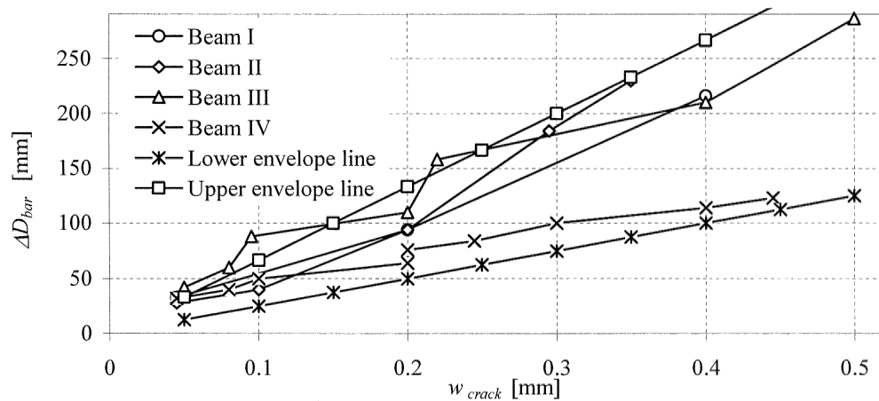
Figure 4. Reduction of rebar diameter \Delta D_{bar} versus the crack width w_{crack} , based on data in Andrade et al. [6].
