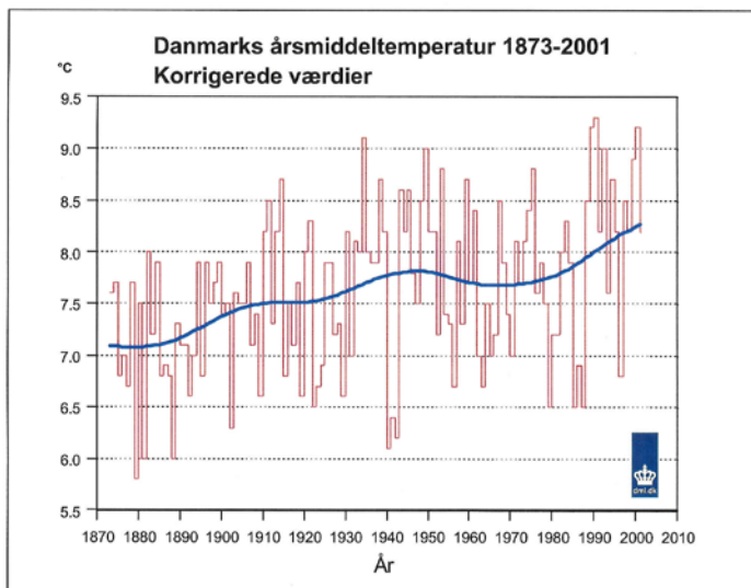
Figure 8. Yearly mean temperatures for Denmark 1873-2001.
