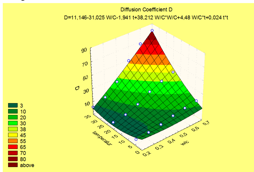
Figure 2. The diffusion coefficient D ( 10^{-12}\text{ m}^2/\text{s} ) as a function of the water-cement ratio w/c and of the temperature \Phi C (Celsius).
