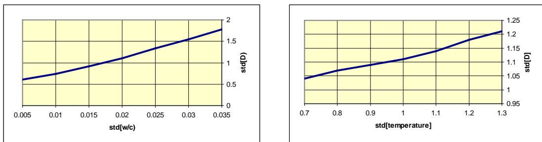
Figure 11. Sensitivity analysis with regard to the standard deviations of w/c and of the temperature.
