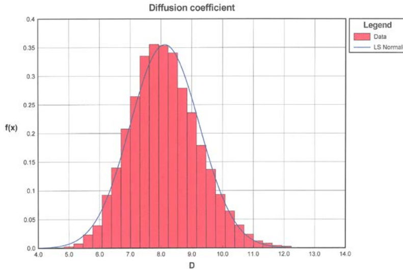
Figure 9. PDF of the diffusion coefficient D ( 10^{-12} \text{ m}^2/\text{s} ).
