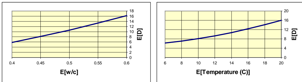
Figure 10 . Sensitivity analysis with regard to the mean values of w/c and of the temperature.
