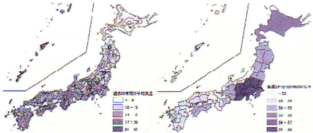
Figure 4. Mean air temperature \Phi and w/c ratio in Japan, figures 3 and 5 in Suda et al. [7].
