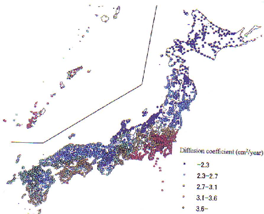
Figure 7. Distribution of the diffusion coefficient D (cm 2 /year) in Japan, figure 15 in Suda et al. [7].
