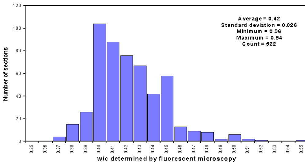
Figure 7. Distribution of w/c measure in 522 thin sections by fluorescence microscopy (Concrete-experts).
