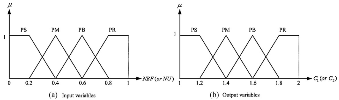
Fig. 3. Membership functions for learning factors fuzzification.
