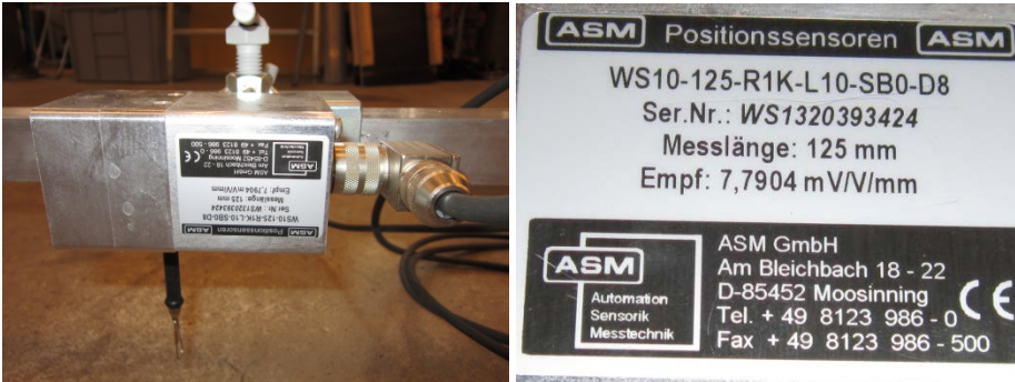
Figure 30: Displacement transducer WS10-2.
