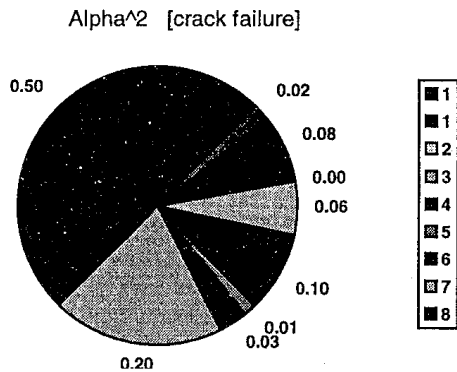
Figure 15: Results of the crack failure analysis. The stochastic variable 8 (model uncertainty) is dominating in this analysis.
