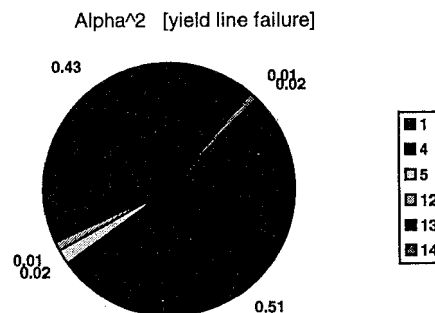
Figure 13: Results of yield line failure analysis. As seen from the "pie" chart the stochastic variables 4 (yield stress of steel) and 13 (HA lane load) are dominating for this failure mode.
