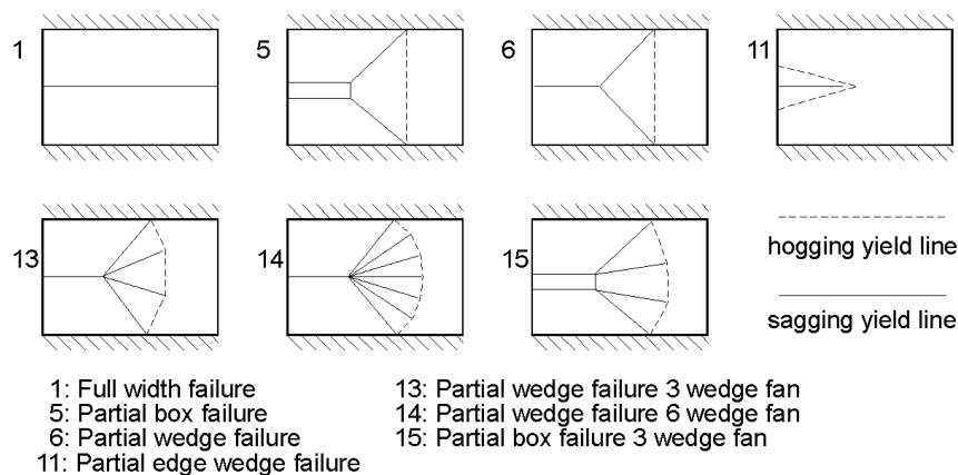
Figure 1. Failure modes for simply supported slab bridges.
