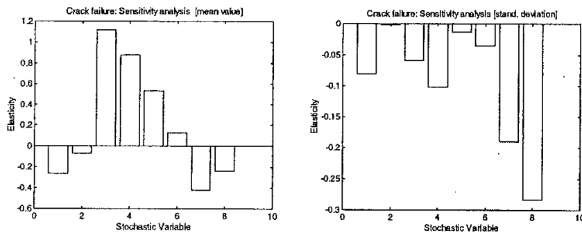
Figure 16: Sensitivity analysis for crack failure.
