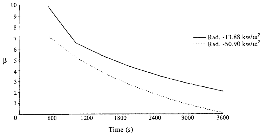
Figure 4. Time-dependent reliability index
