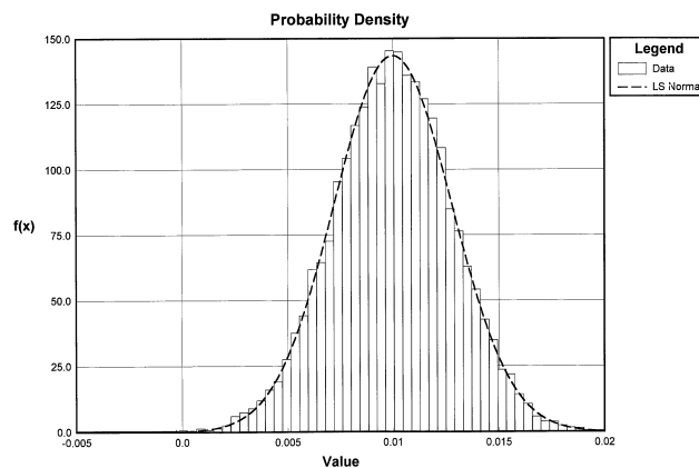
Figure 6. Stochastic modelling of W_{crit} .
