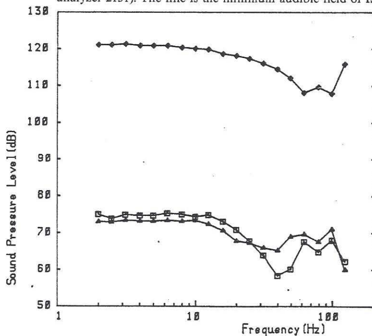
Fig 4. Frequency response and harmonic distortion from the loudspeakers for a fixed output voltage from the power amplifier. The measurement point was in the centre of the room. (◇) fundamental, (□) second harmonic, (Δ) third harmonic.
