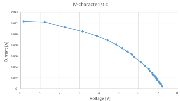
Figure 11: The IV-characteristic of the solar cell
