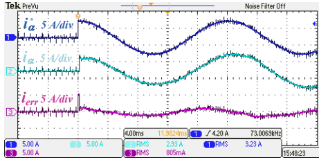
Fig. 21. Step response – P controller with lead compensator: k_{pl} = 11.56 , k_{li} = 0.475 , reference (5 A/div), real (5 A/div) and inductor current error (5 A/div) ( \alpha -axis), time scale (4 ms/div)
