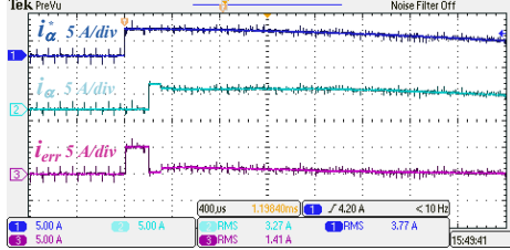
Fig. 22. Step response – P controller with lead compensator: k_{pl} = 16.82 , k_{li} = 0.868 , reference (5 A/div), real (5 A/div) and inductor current error (5 A/div) ( \alpha -axis), time scale (400 \mu s/div)
