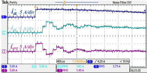
Fig. 18. Step response – P controller: k_{pI} = 16.82 , reference (5 A/div), real (5 A/div) and inductor current error (5 A/div) ( \alpha -axis), time scale (400 \mu s/div)
