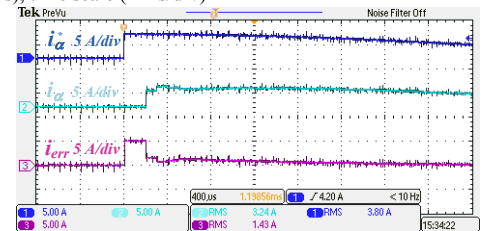
Fig. 20. Step response – P controller with lead compensator: k_{pI} = 16.82 , k_L = 0.868 , reference (5 A/div), real (5 A/div) and inductor current error (5 A/div) ( \alpha -axis), time scale (400 \mu s/div)
