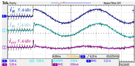
Fig. 15. Step response – P controller: k_{pI} = 11.56 , reference (5 A/div), real (5 A/div) and inductor current error (5 A/div) ( \alpha -axis), time scale (4 ms/div)
