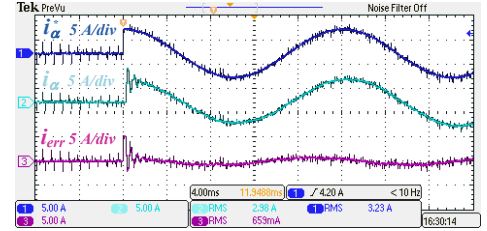
Fig. 17. Step response – P controller: k_{pI} = 16.82 , reference (5 A/div), real (5 A/div) and inductor current error (5 A/div) ( \alpha -axis), time scale (4 ms/div)
