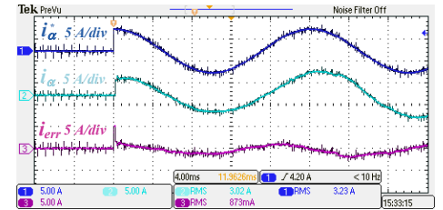
Fig. 19. Step response – P controller with lead compensator: k_{pI} = 11.56 , k_L = 0.475 , reference (5 A/div), real (5 A/div) and inductor current error (5 A/div) ( \alpha -axis), time scale (4 ms/div)
