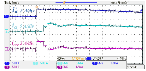
Fig. 16. Step response – P controller: k_{pI} = 11.56 , reference (5 A/div), real (5 A/div) and inductor current error (5 A/div) ( \alpha -axis), time scale (400 \mu s/div)
