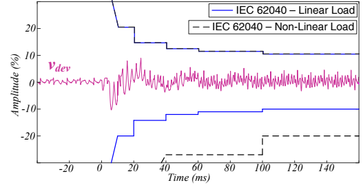
Fig. 26. Nonlinear step load changing (0 – 100%): Dynamic characteristics according to IEC 62040 standard for linear loads: overvoltage ( v_{dev} > 0 ) and undervoltage ( v_{dev} < 0 )
