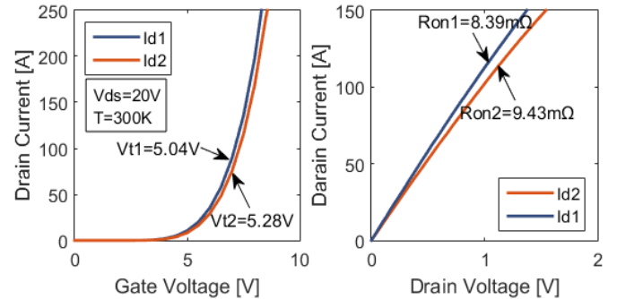
Fig. 18. Mismatch between the static characteristics for two Cree 1.7kV modules
