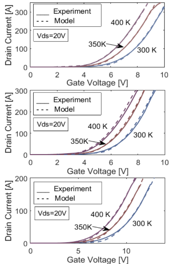
Figure 8. I_d - V_{gs} validation with temperature spread for three modules: Cree (top), Microsemi (middle), Rohm (bottom).
