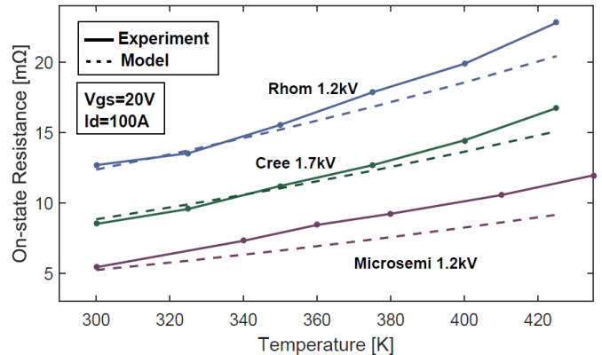
Fig. 10. R_{on} variation with temperature for three modules with model validation
