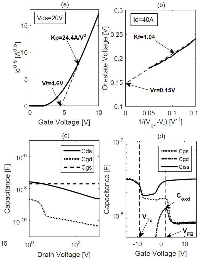
Fig. 3. Parameter extraction sequence: (a) saturation region; (b) linear region; (c)-(d) transient parameters
