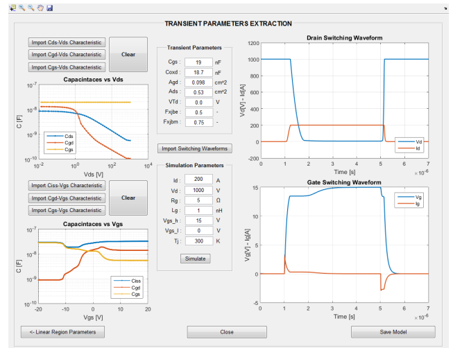
Fig. 6. MATLAB GUI panel for the identification of the transient parameters
