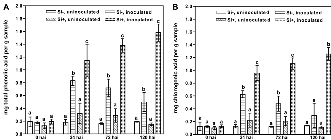
Figure 2. Contents of total phenolic acids (A) and 5-O-caffeoylquinic acid (chlorogenic acid; B) in leaf extracts of rose from plants either treated with (Si+) or without (Si-) Si followed by either inoculation with P. pannosa or no inoculation. Data represent results from one experiment, and each observation represents the mean from three extractions. All values are presented as means \pm SE. Means within each time point are comparable, and bars marked by different letters are significantly different. Further information on the results from this experiment is given in Supplemental Table S1. The findings of this experiment were confirmed in a second independent experiment.
