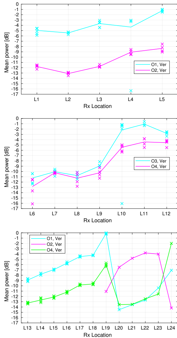
Fig. 7. Mean total power for different Tx antenna orientations and locations in the Lab (top), Corridor (middle), and Hall (bottom) environment. All values are normalized to the maximum observed in the Hall environment.
