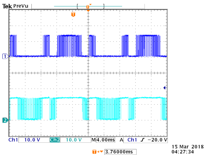
(e) Ch1: S_1(t) : 10 V/Div; Ch2: S_2(t) : 10 V/Div
