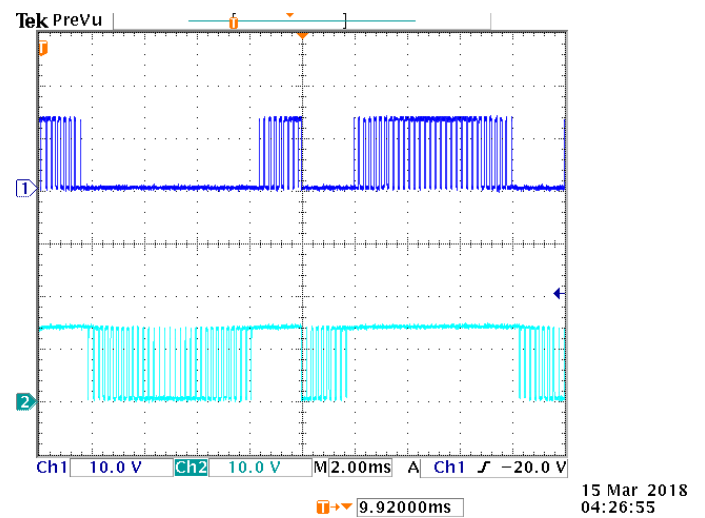
(f) Ch1: S_1(t) : 10 V/Div; Ch2: S_2(t) : 10 V/Div
