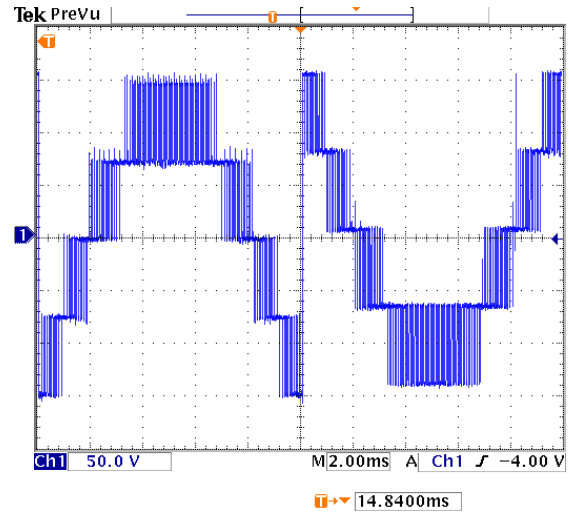
(b) Ch1: v_{An}(t) : 50 V/Div
