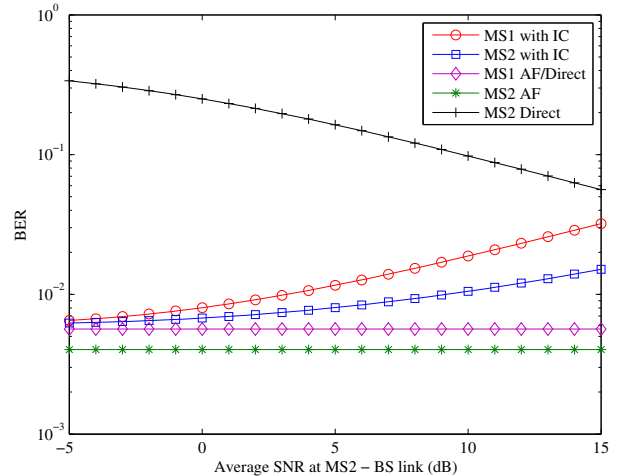
Fig. 5. BER against average SNR at MS2-BS link when average SNR at MS1-BS link is set to 35 [dB], MSs-RS links to 40 [dB], and RS-BS link to 50 [dB].
