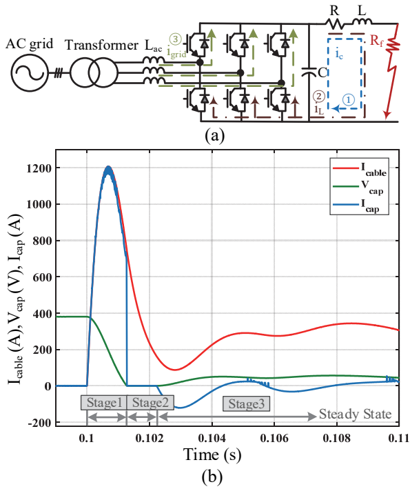
Fig. 3. (a) Equivalent scheme of VSC under a short-circuit fault, (b) Cable current i_{cable} , DC-link capacitor voltage V_{cap} , and capacitor current I_{cap} during the short-circuit fault.
