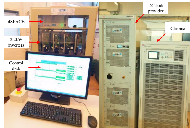
Fig. 17. Experimental setup.
