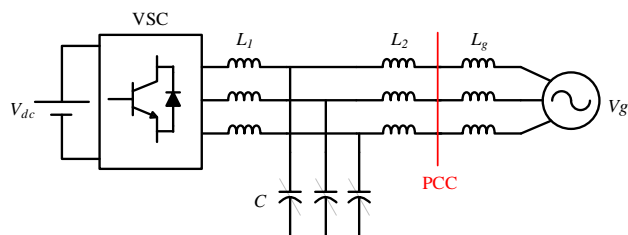
Fig. 1. Typical three phase grid-connected inverter with LCL filter.
